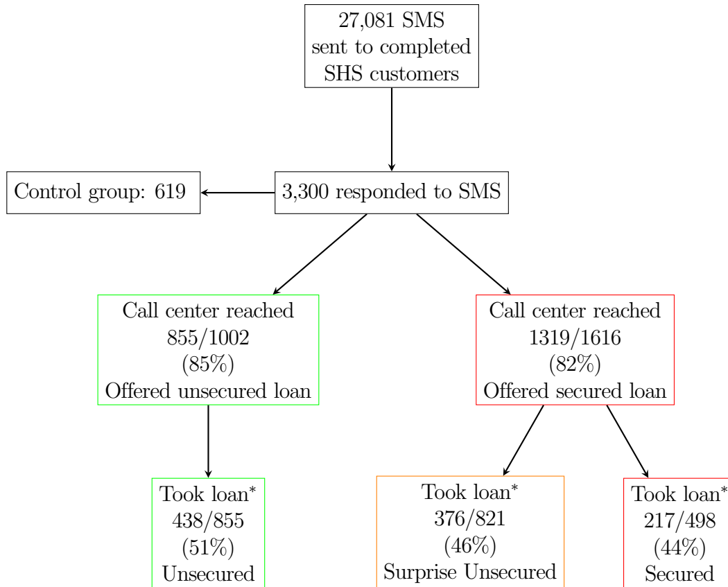
Figure 3: Experimental Design
